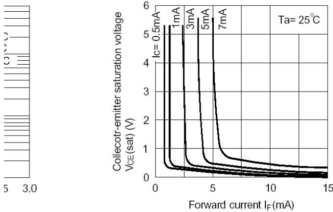
Fig.3 Collector-emitter Saturation Voltage vs. Forward Current
