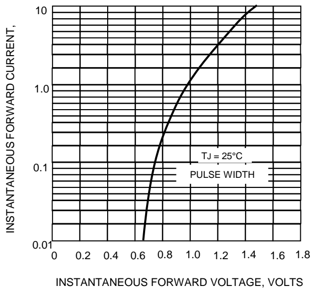
FIG.4-TYPICAL FORWARD CHARACTERISTICS
