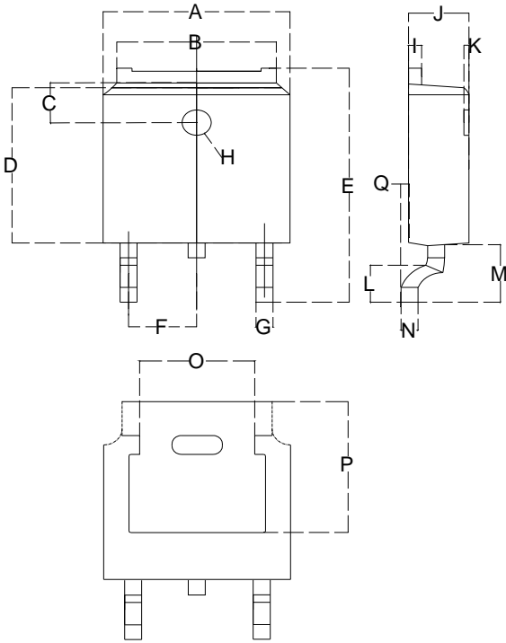
TO-252
