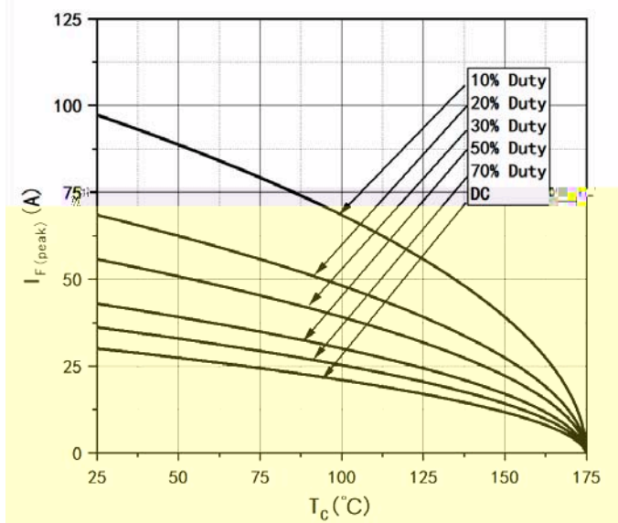
Figure 7. Current Derating
